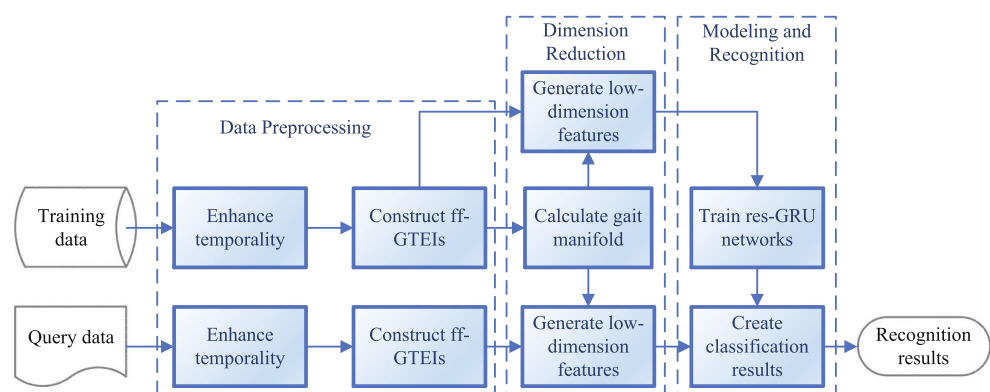
Fig. 1 Flow chart of the proposed human identification framework
