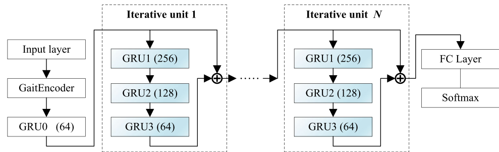
Fig. 5 The proposed residual gated recurrent unit network model
