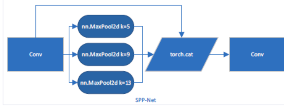
Figure 2: SPP-Net
