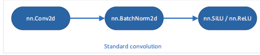
Figure 1: Conv model
