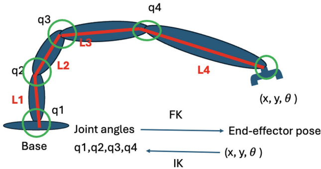
Fig. 2.18 The comparison between FK and IK
