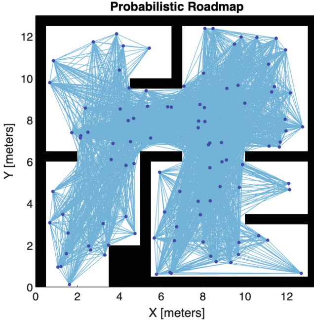
Fig. 2.10 An example of PRM algorithm
