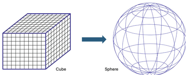
Fig. 7.3 From cube to sphere
