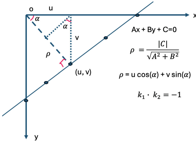
Fig. 3.10 Hough transform
