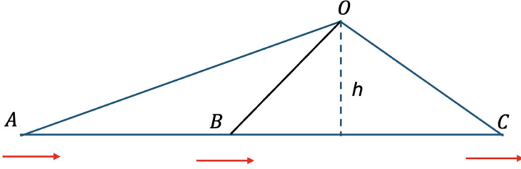
Fig. 2.12 A triangulation for surveying
