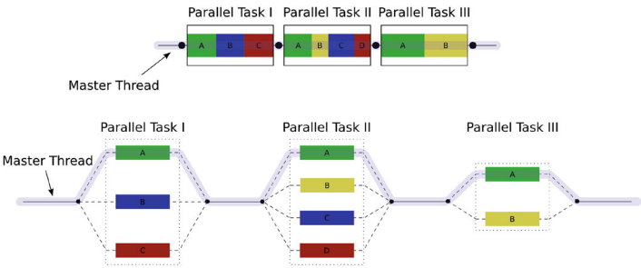
Fig. 8.2 Fork-join model
