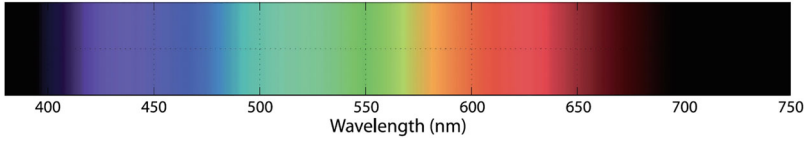
Fig. 3.1 The visible spectrum
