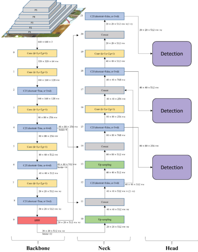
Fig. 2. The architecture of YOLOv8 model
