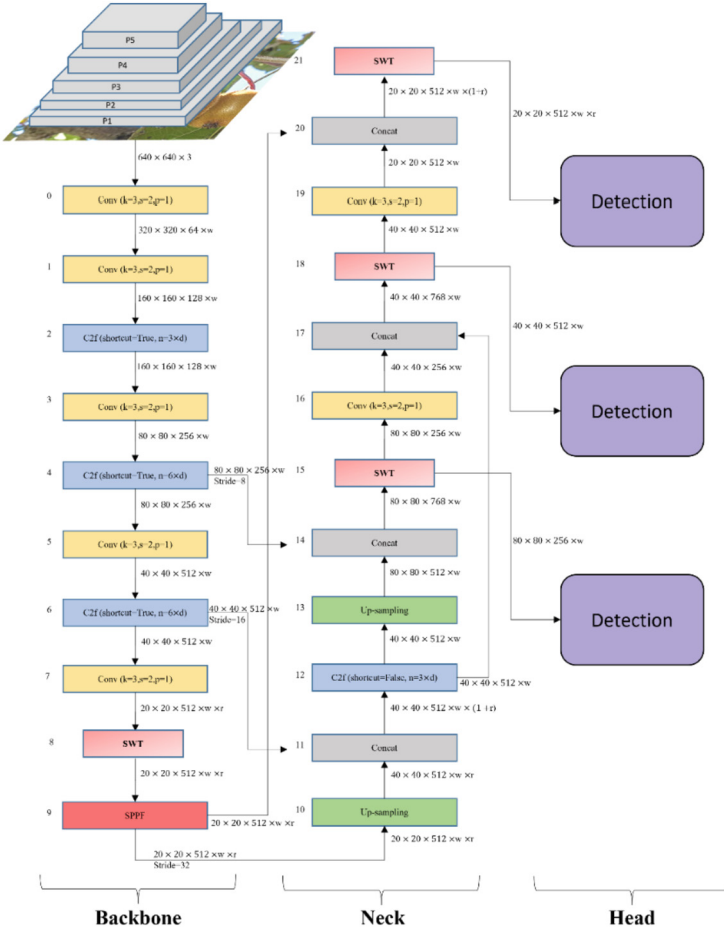
Fig. 3. The architecture of enhanced Kiwifruit detection model
