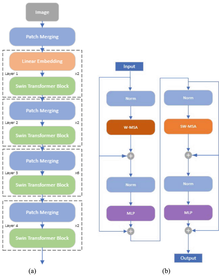
Fig. 1. The architecture of Swin Transformer
