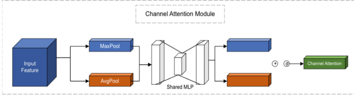
Fig. 3. The structure of channel attention module.
