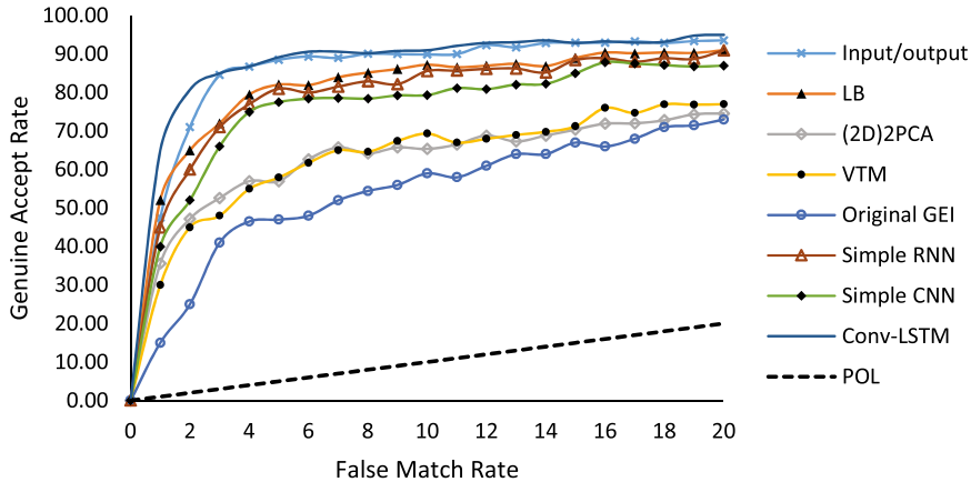
Fig. 5. The ROC curves of the methods based on CASIA dataset B.
