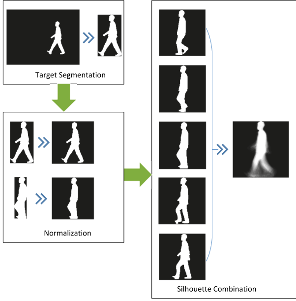
Fig. 2. The diagram of Conv-LSTM-based gait recognition.
