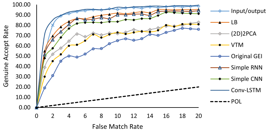
Fig. 6. The ROC curves for gait recognition methods based on OU-ISIR LP.
