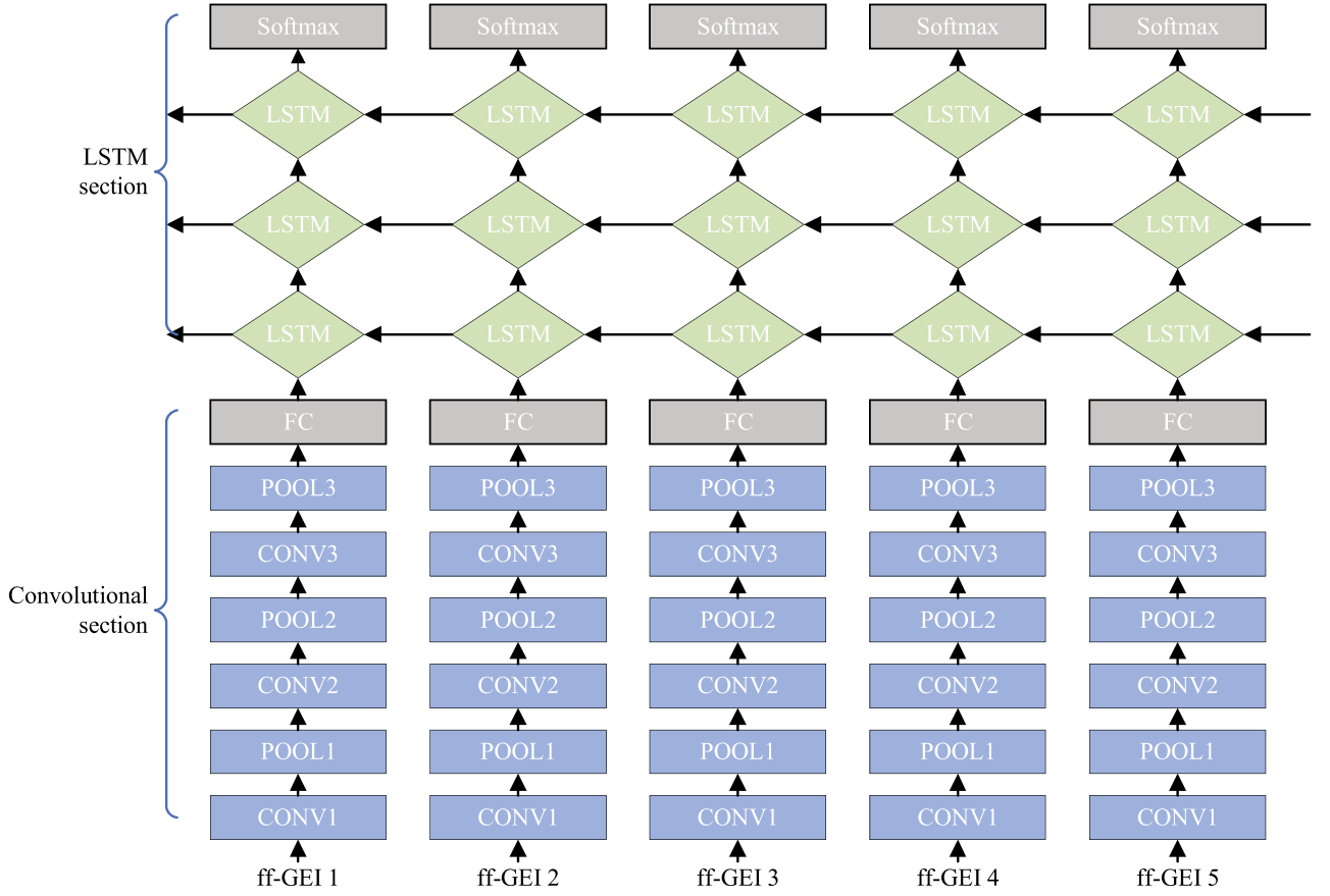
Fig. 3. The architecture of the proposed gait recognition network based on Conv-LSTM.
