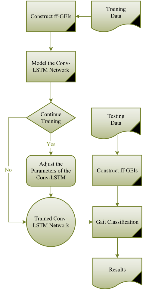
Fig. 1. The diagram of Conv-LSTM-based gait recognition.
