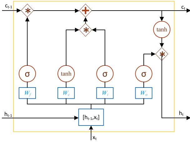
Fig. 4. The diagram for one LSTM layer in Conv-LSTM.
