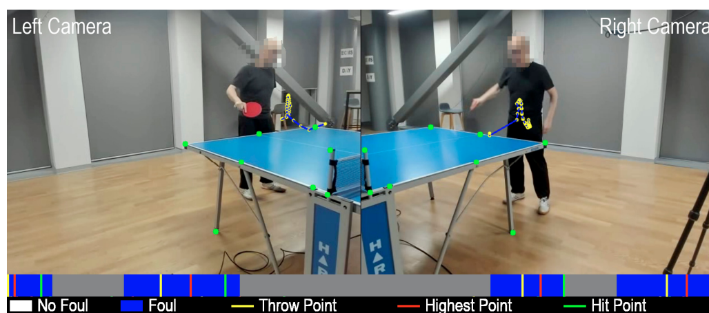
Figure 9. Video Segmentation Results: (Top) Synchronized left and right camera views showing key trajectory points during a table tennis serve. The throw point (yellow), highest point (red), and hit point (green) are marked to track the ball's trajectory. (Bottom) Segmented timeline showing frame classification as “No Foul” (gray) and “Foul” (blue), with transitions aligned to the serve events.
