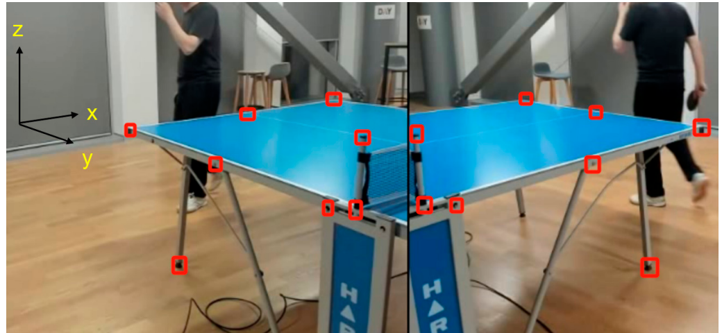
Figure 3. The calibration points are applied to align cameras with a coordinate system. The 16 fixed reference points are labeled with their 3D coordinates in the image, providing the foundation for accurate spatial calibration.
