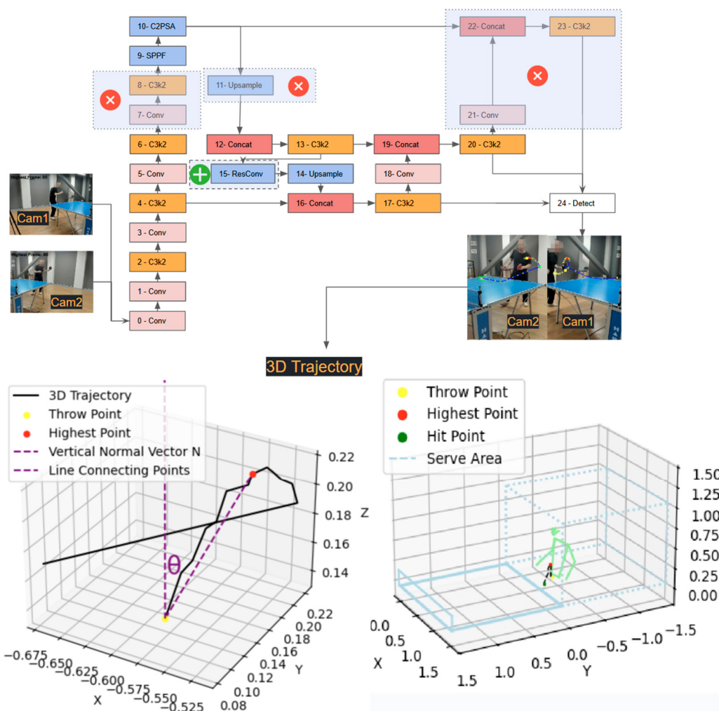
Figure 4. Modified YOLOv11 architecture for small object detection. The large object detection layer is removed, and a Custom ResConv layer is added to enhance detection performance for small, fast-moving objects like the table tennis ball.
