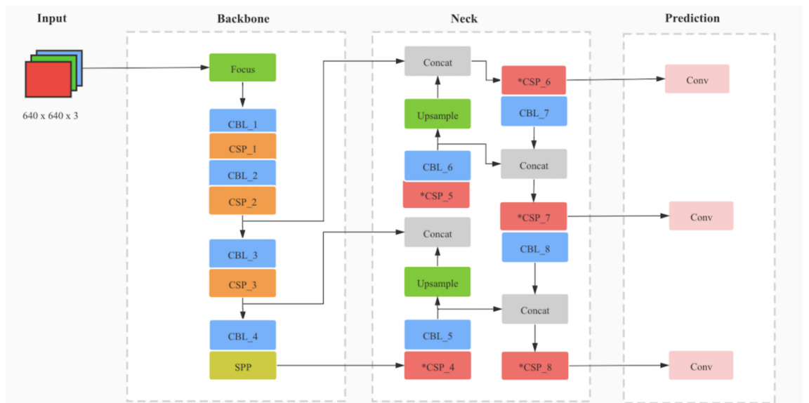
Figure 3.5 The architecture of YOLOv5
