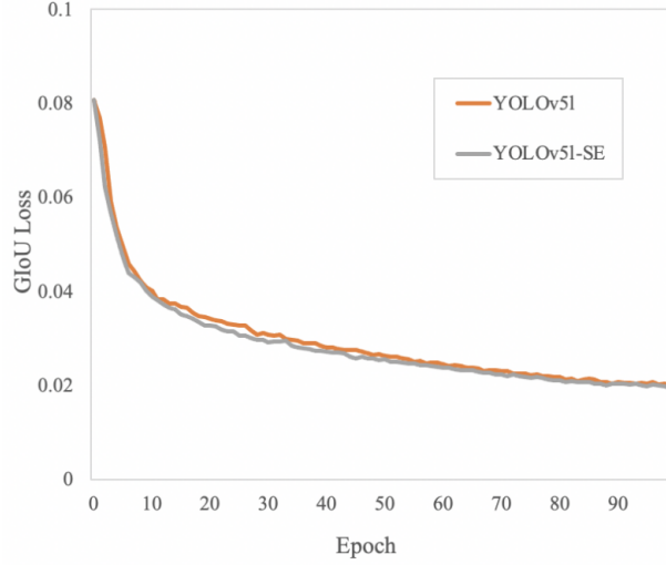
Figure 4.5 The GloU loss in different epochs
