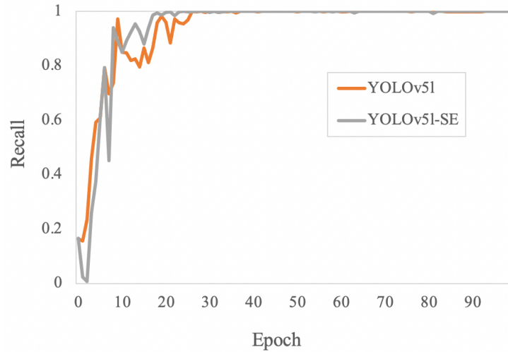
Figure 4.4 The recall in different epochs
