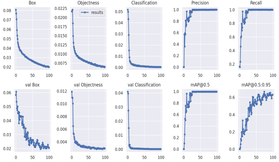
Figure 4.1 The measure of loss and precision for YOLOv5l
