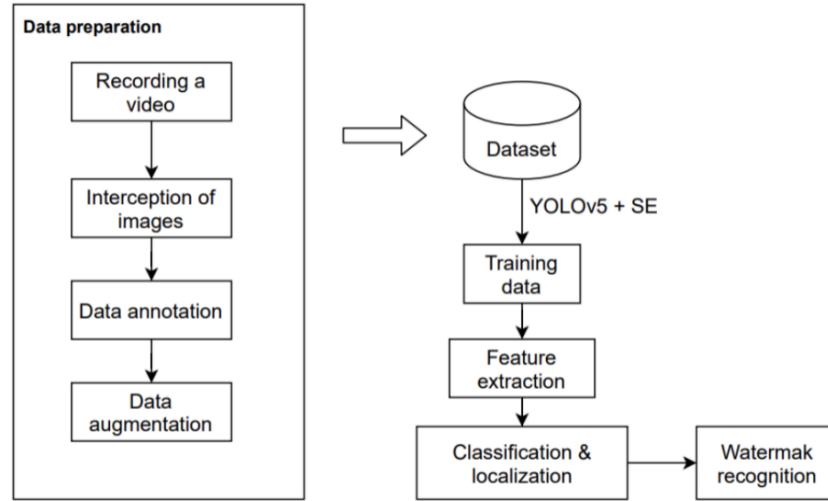
Figure 3.1 The phases of the experiment
