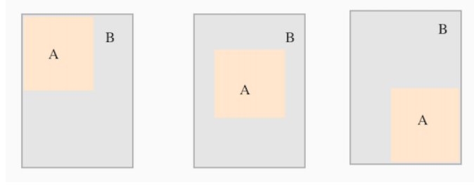
Figure 3.7 The degeneration of GIoU
