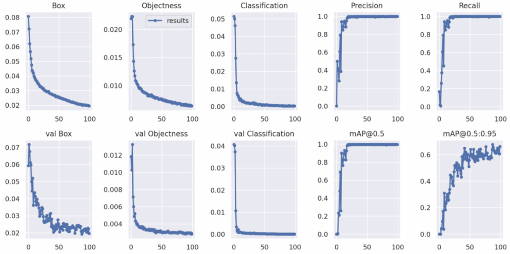
Figure 4.2 The measure of loss and precision for YOLOv5l-SE
