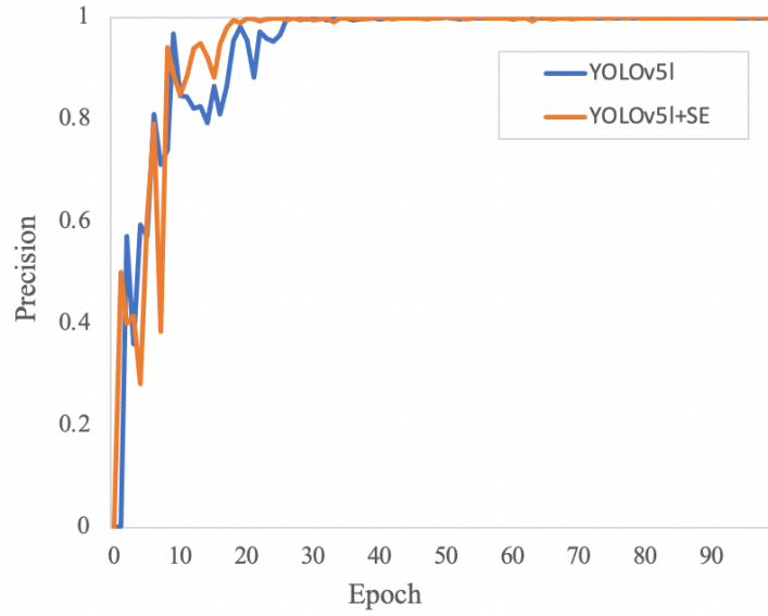
Figure 4.3 The precision in different epochs
