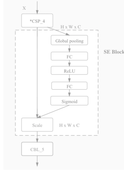
Figure 3.8 The architecture of SE block in YOLOv5
